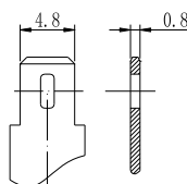
Terminal T1
