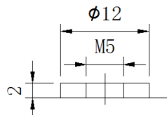
Terminal T8
