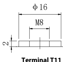
Terminal T11
