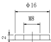
Terminal T11
