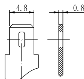
Terminal T1
