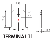
TERMINAL T1
