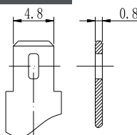
Terminal T1
